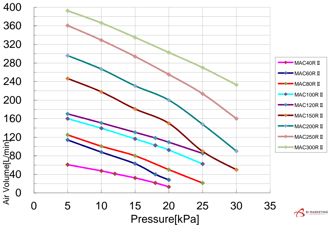
FujiMAC Series Performance Curve -230V50Hz MAC40R II / 60R II / 80R II / 100R II / 120R II / 150R II / 200R II / 250R II / 300R II
